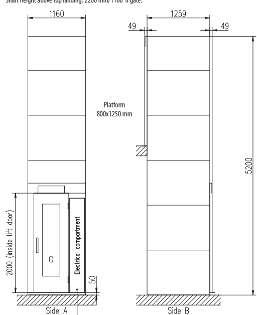
Shaft height above top landing: 2200 mm/1100 if gate.
